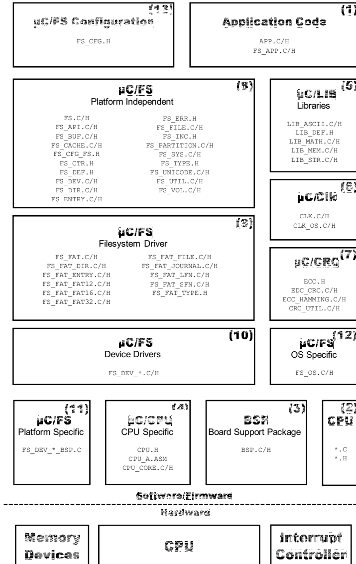
Figure 3-1 µC/FS Architecture
