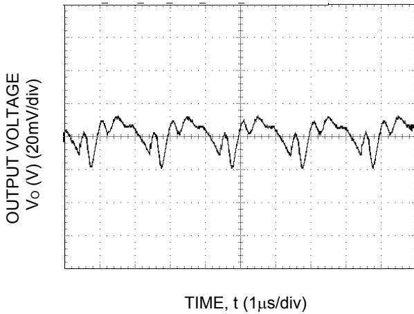
Fig-41. Typical output ripple and noise (CO=2x47µF ceramic, VIN = 12V, Io = Io,max, ).
